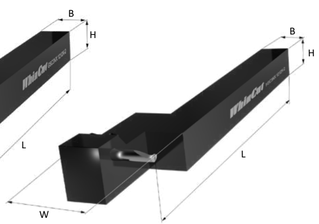
HSC | Square shanks with centreline at top
