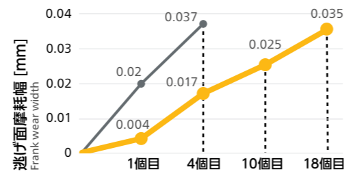
逃げ面摩耗幅の推移 Frank wear progress
